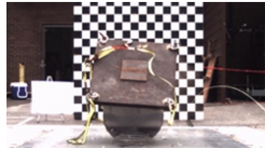
Drop Test
